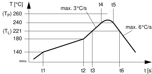
Illustration 5: Soldering profile
